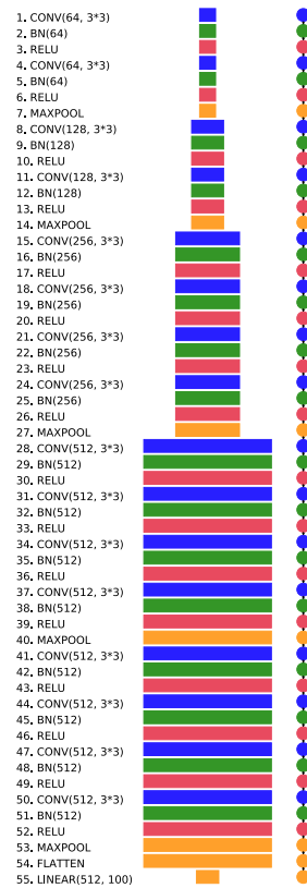
Teacher: VGG-19
