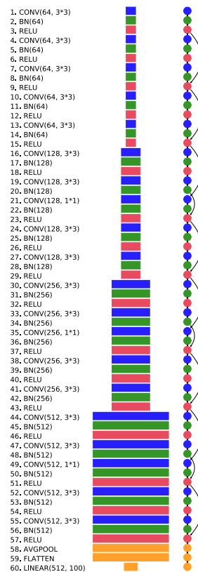
Teacher: ResNet-18
