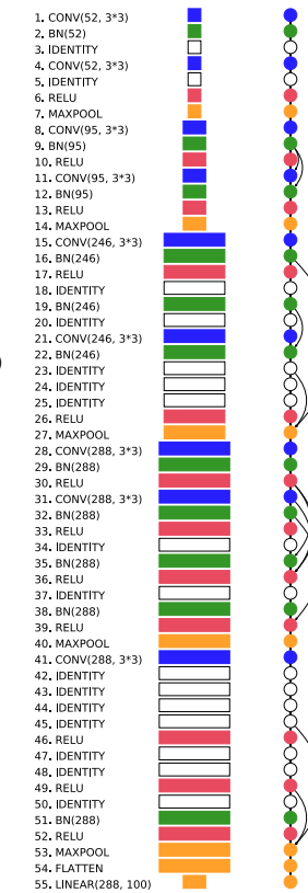
Compressed on CIFAR-100
